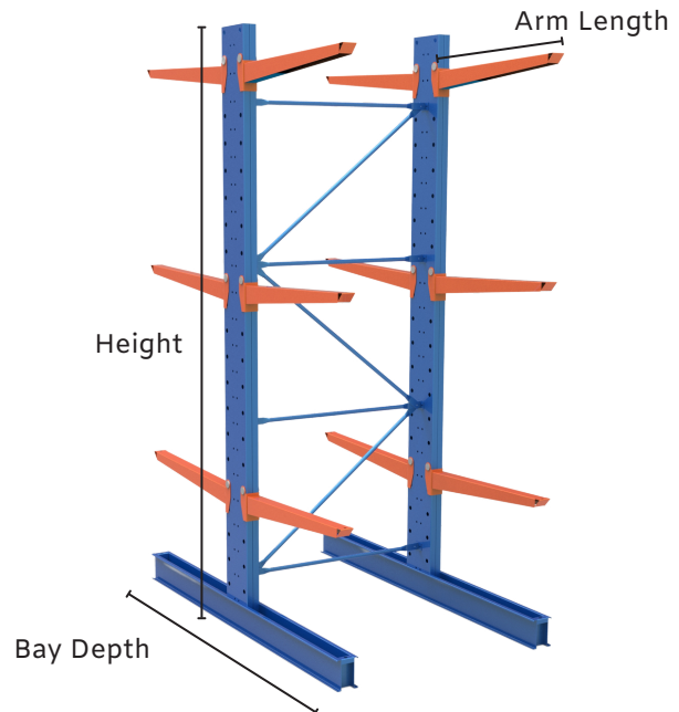
DOUBLE SIDED
